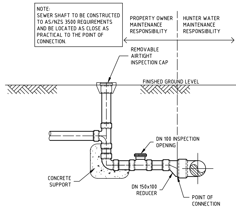
TYPICAL NON-BOUNDARY TRAP SEWER SHAFT- RESIDENTIAL
