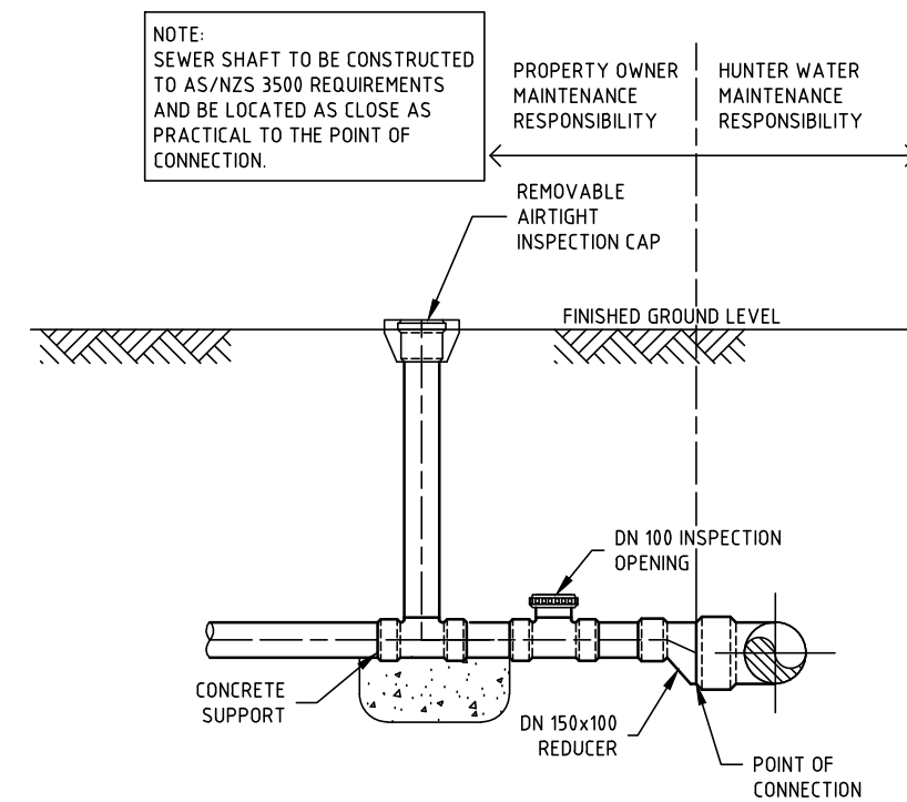
TYPICAL NON-BOUNDARY TRAP (SHALLOW CONNECTION) INSPECTION SHAFT- RESIDENTIAL
