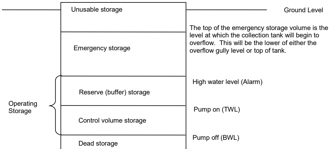
Figure 1: Storage Components of a PSS Collection Tank
