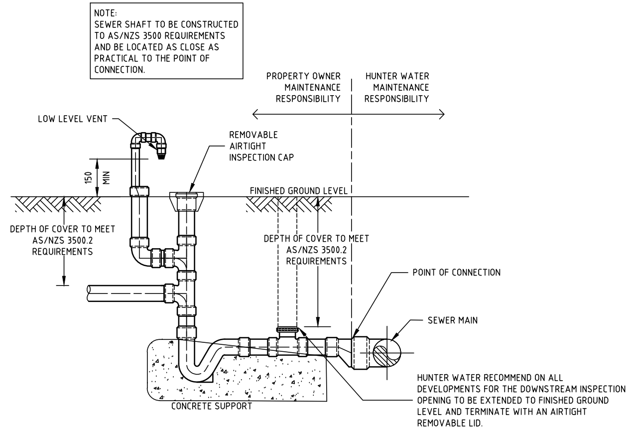
TYPICAL BOUNDARY TRAP SEWER SHAFT - RESIDENTIAL
