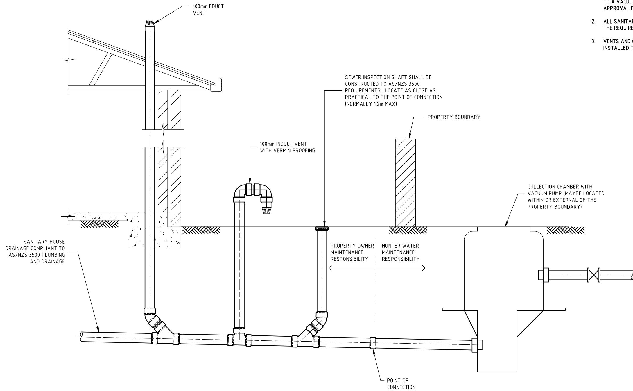
TYPICAL VACUUM SEWER SYSTEM
