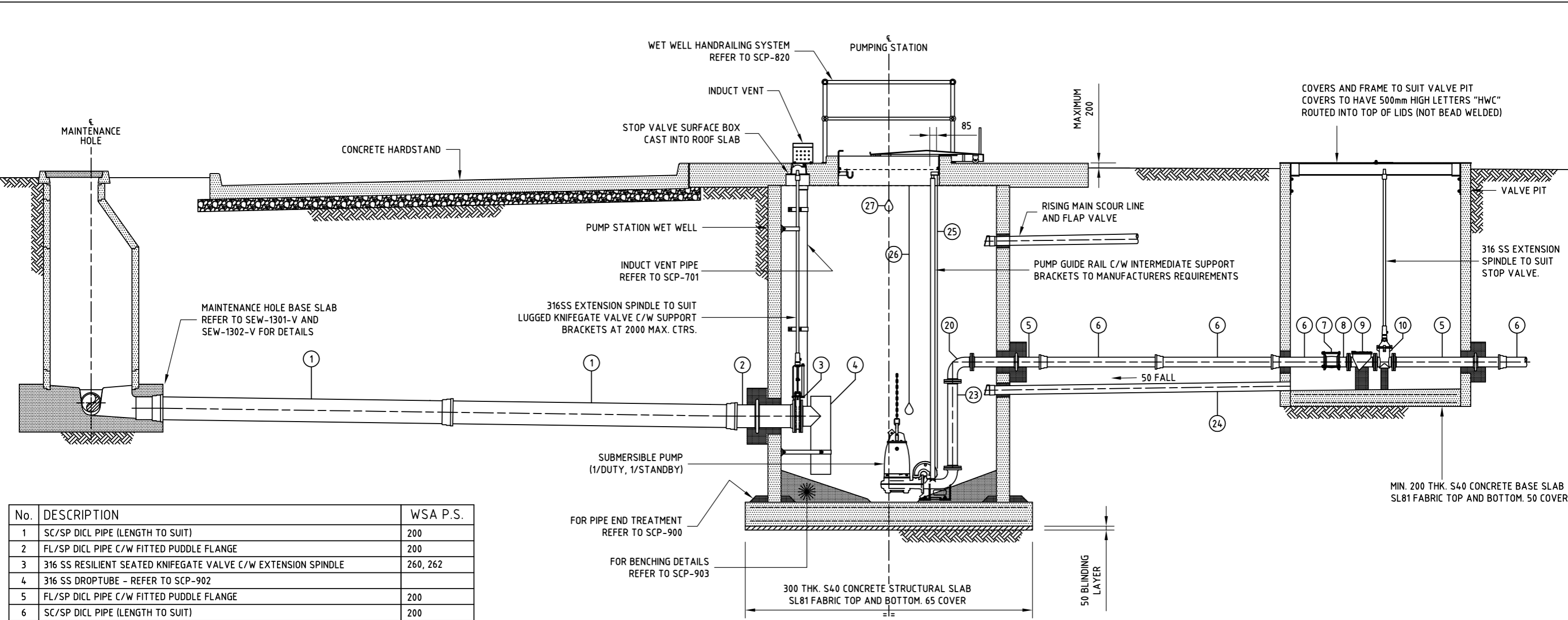
SECTIONAL ELEVATION SCALE 1: 50
