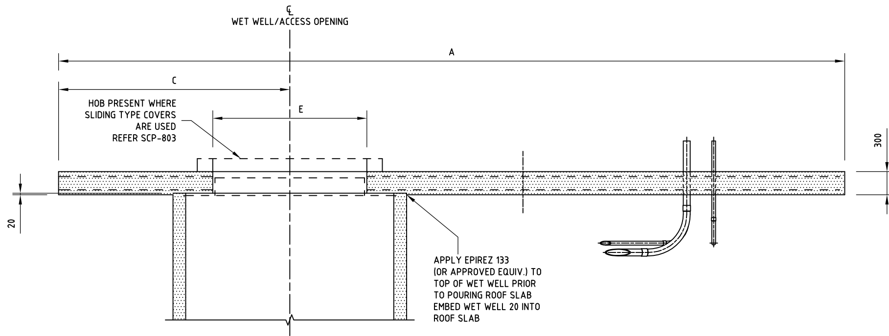
SECTION A 700 SCALE 1:50
