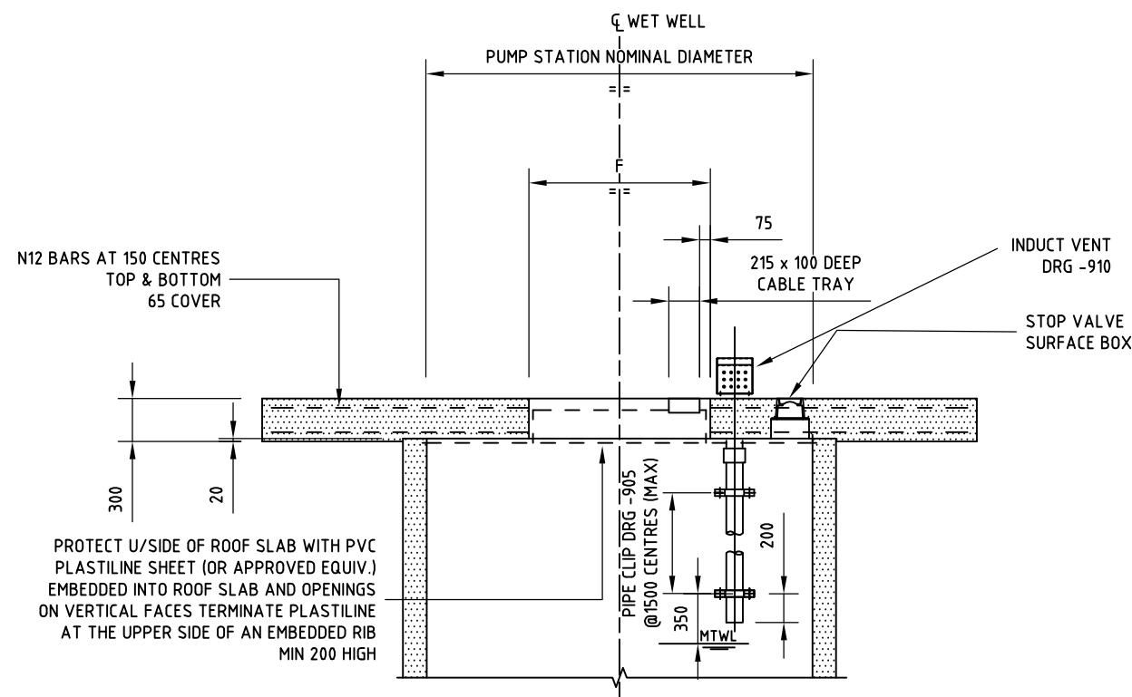
SECTION B 700 SCALE 1:50
