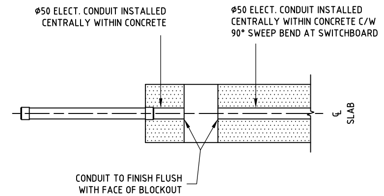
ENLARGED SECTION C 700 SCALE 1:20
