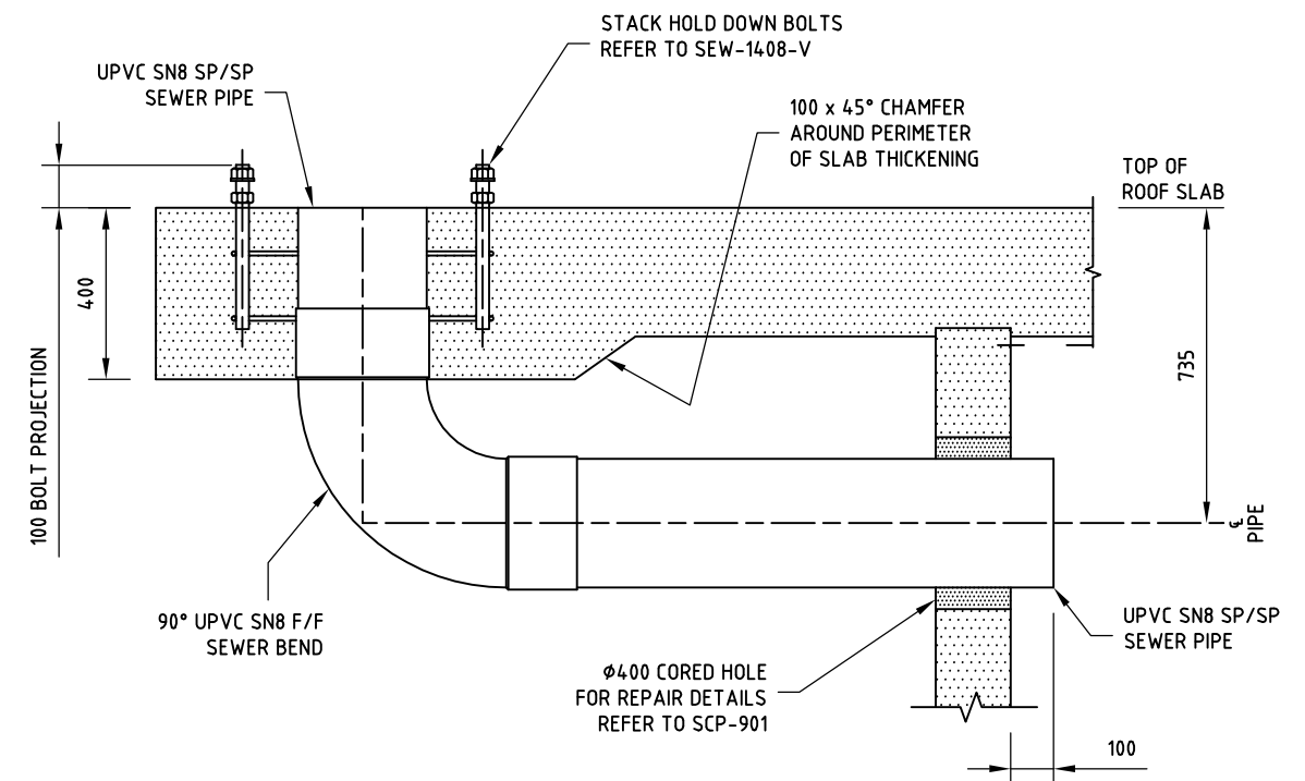
ENLARGED SECTION D 700 SCALE 1:20
