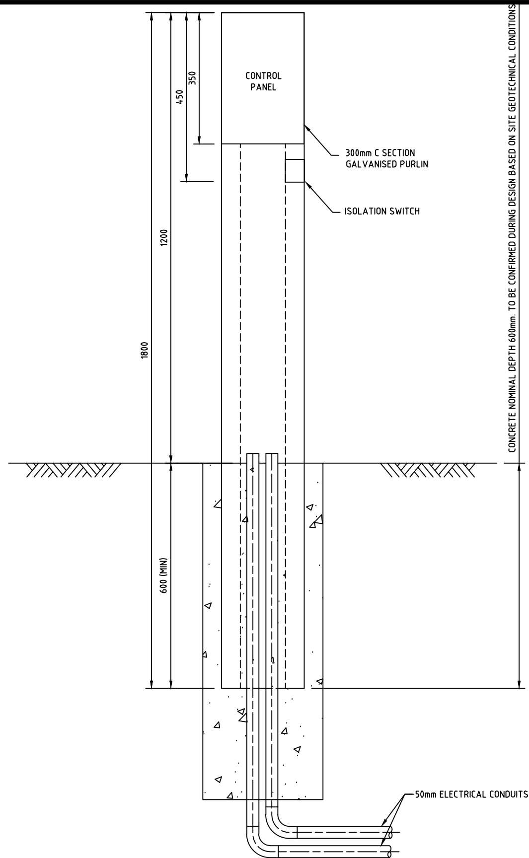
TYPICAL CONTROL PANEL MOUNTING POST
