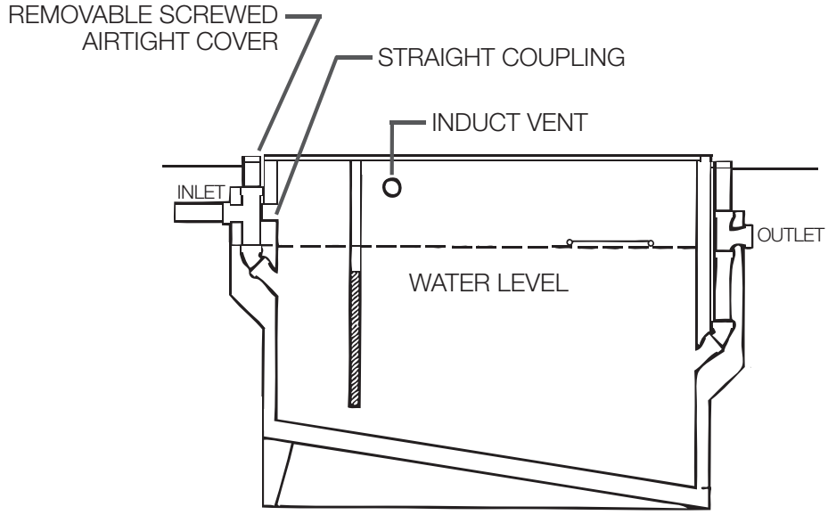
SECTION ELEVATION
